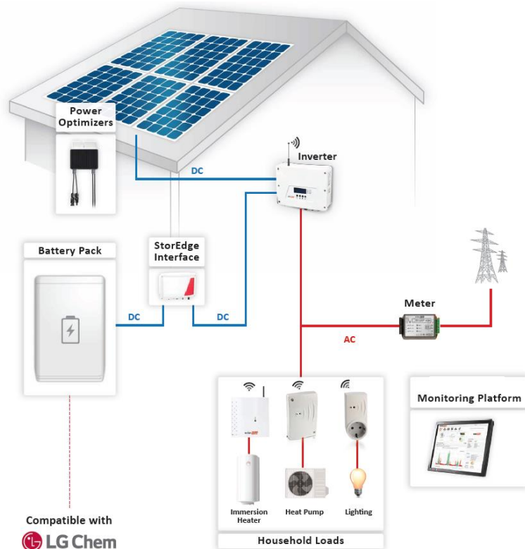
Figure 1: Smart Energy - system overview
