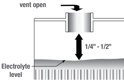
Figure 7 – Electrolyte level
