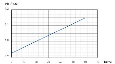
Corrective factor for power losses vs. ambient temperature
